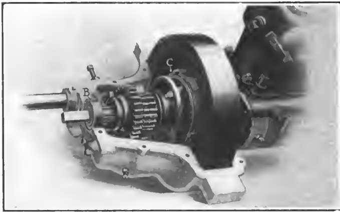
Fig. 9—Showing the simplicity of the clutch and transmission
